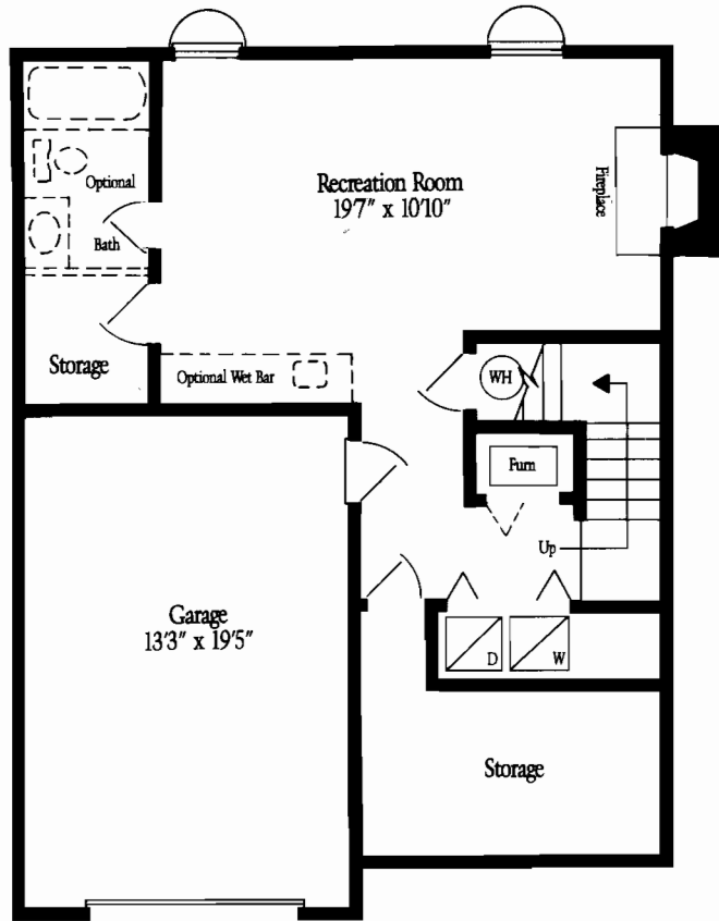
Basement Level with Garage
